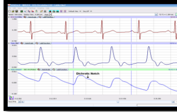
ECG signal
